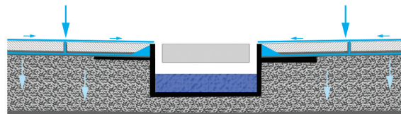
Cross section of linear drain
