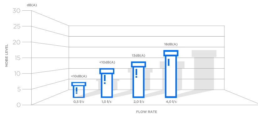
Noise level of the PEŠTAN S LINE system in accordance with VDI 4100
