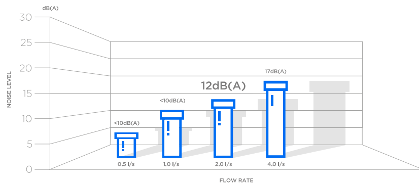
Noise level of the PEŠTAN S LINE system in accordance with EN 14366
