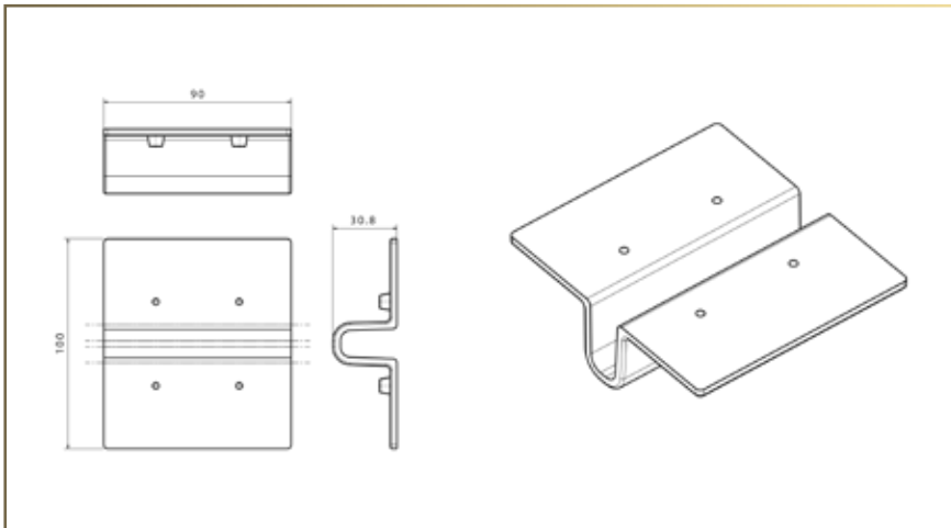
Straight connector
