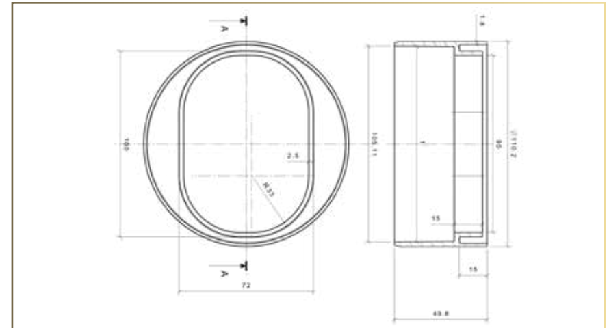
Rubber ring
