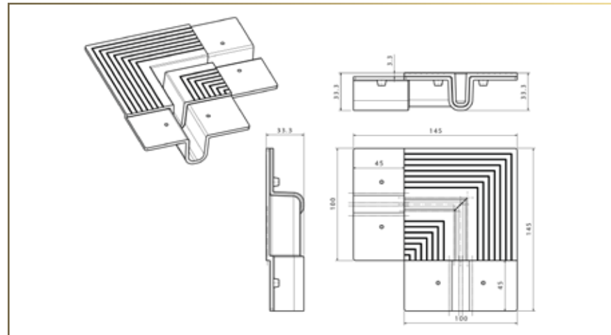
Corner connector
