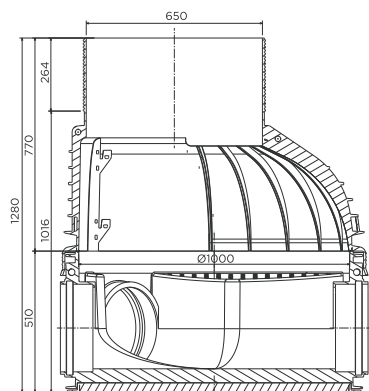
minimum height manhole
