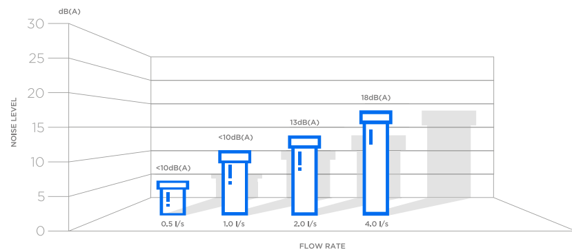
Noise level of the PESTAN S LINE system in accordance with VDI 4100
