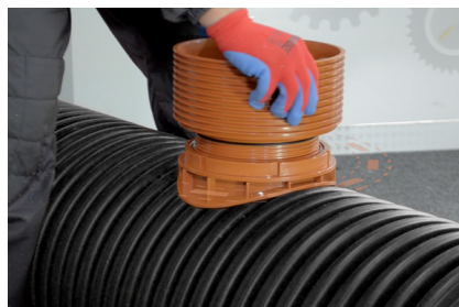
11. Setting the selected connection
